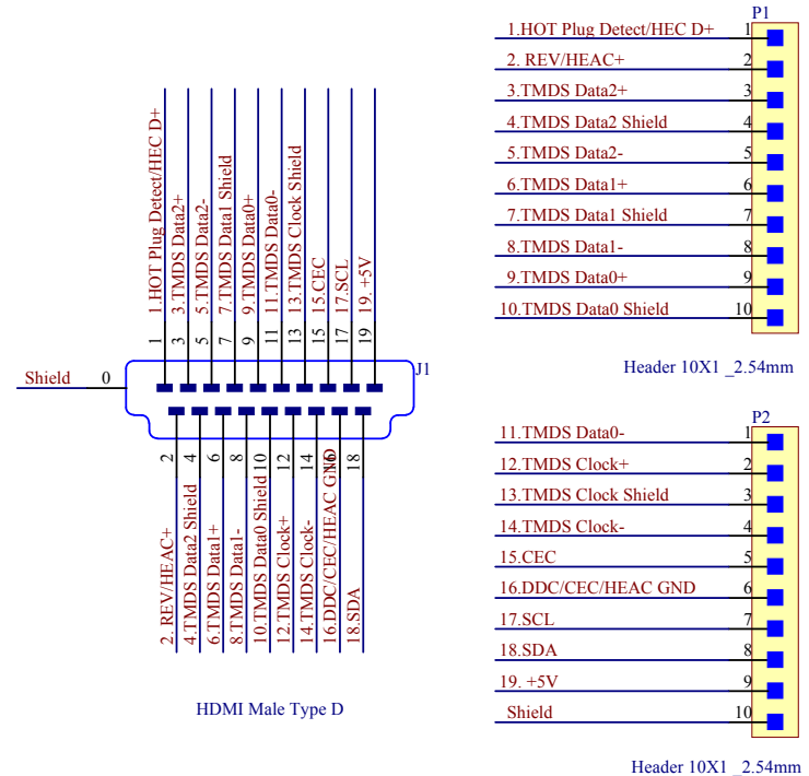
HDMI-DM-BO-V1A Schematic Diagram
